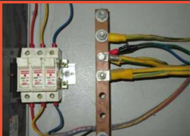
Multi looping of cables
